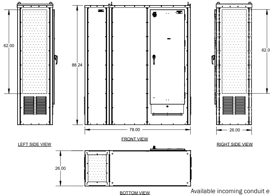
Available incoming conduit entry locations shown shaded
