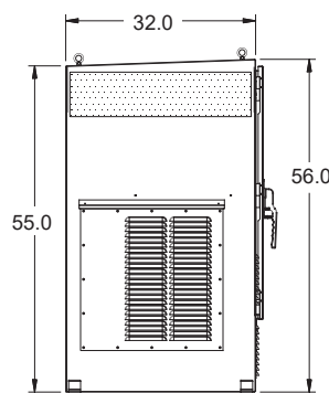
LEFT VIEW
